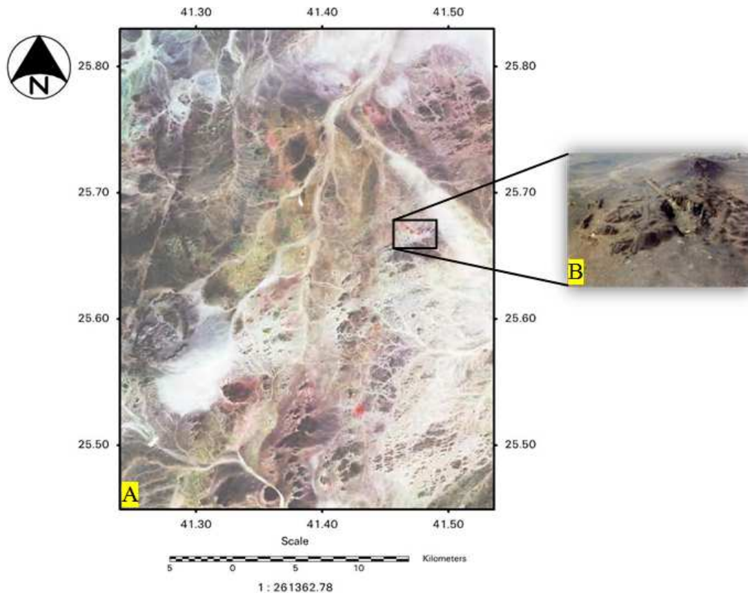
Figure 3. SWIR Color Composite (BANDS 469-RGB) in 3-A and Field Photograph in 3-B.
