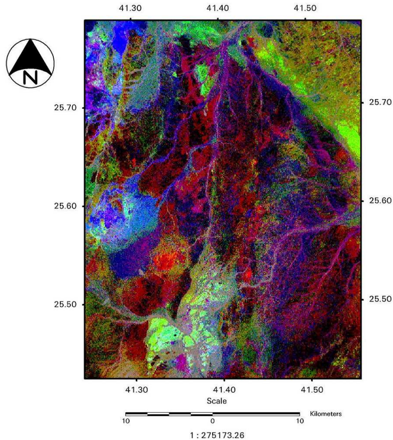
Figure (3): Colore composite of ratio images 1/2, 4/5 and 7/5 (RGB) Prepared from ASTER, Showing Gossan in Bright Red, while Areas of Hydrothermal alteration from pink to red.
