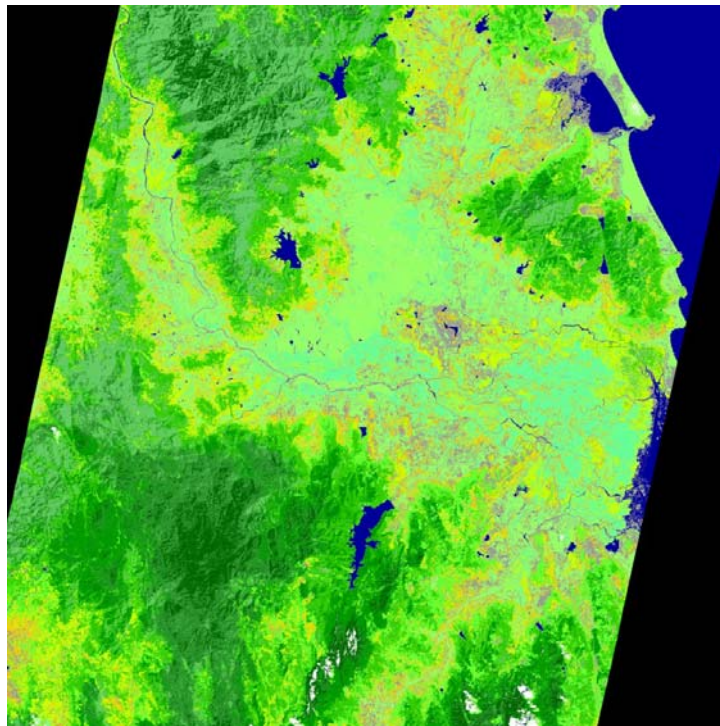
Fig. 8 Landcover extracted from 14 bands of ASTER
