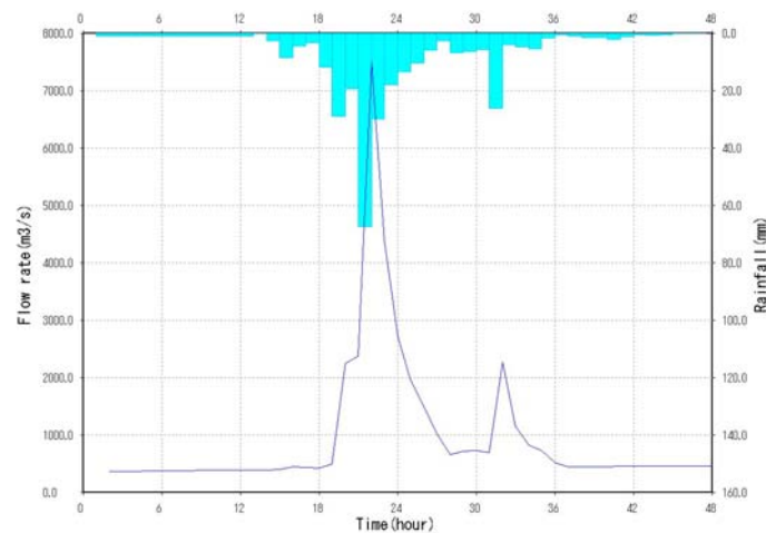
Fig. 9 Hyeto-hydrograph calculated by runoff simulation
