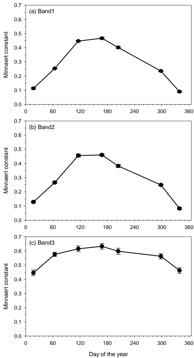
Fig. 5. The Minnaert constants derived from stratified random sampling, Sample II. Error bars represent standard deviations. (a) Band 1, (b) Band 2, and (c) Band 3.
