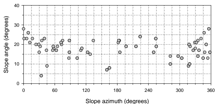
Fig. 2. Scattergram between slope azimuth and slope angle for the analysis of Sample I.
