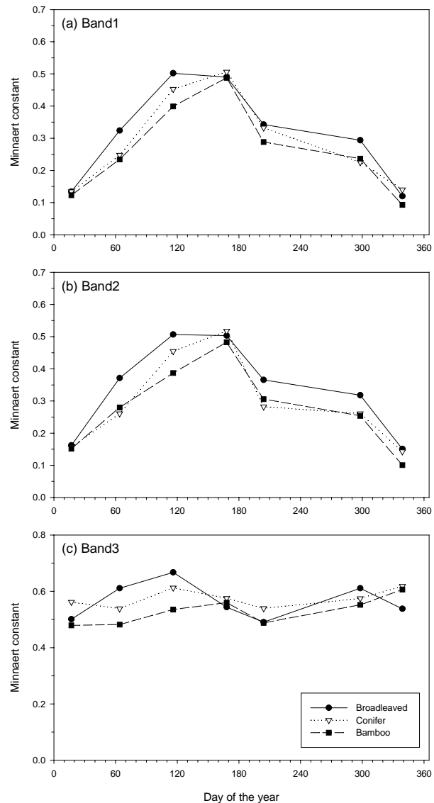
Fig. 3. The Minnaert constants for three forest types derived from same topographical features. (a) Band 1, (b) Band 2, and (c) Band 3.
