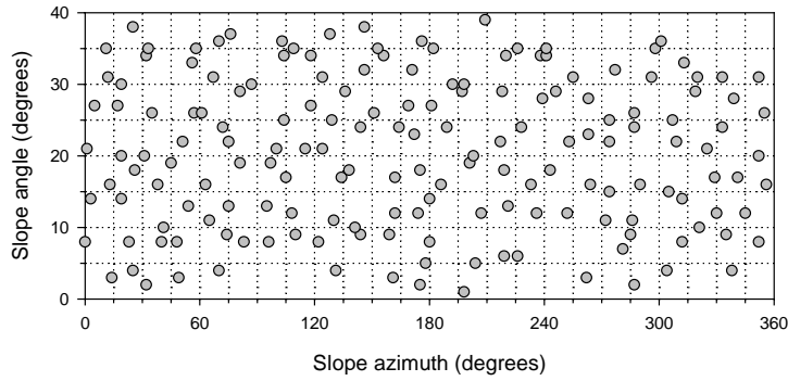
Fig. 4. Scattergram between slope azimuth and slope angle for the analysis of Sample II.
